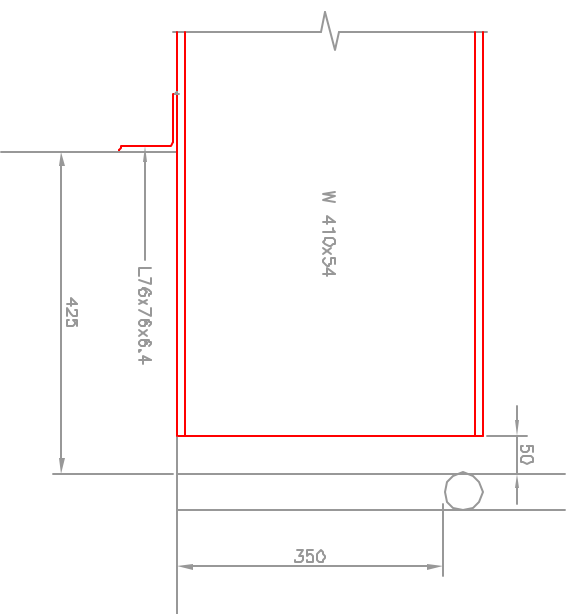
DETAIL 'B' 1:10
