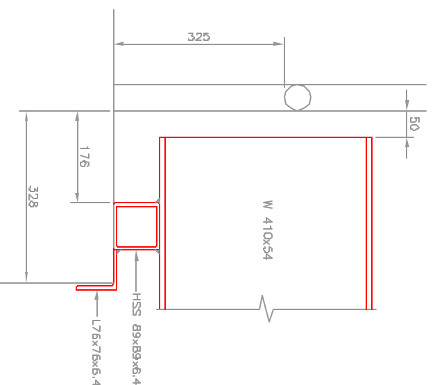
DETAIL 'A' 1:10
