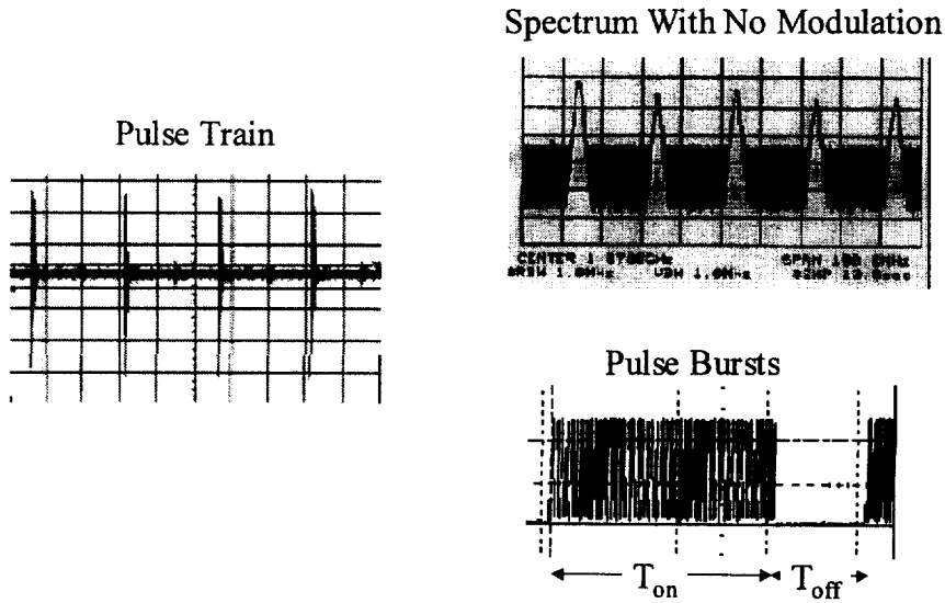
Figure 2: Different UWB Signals
