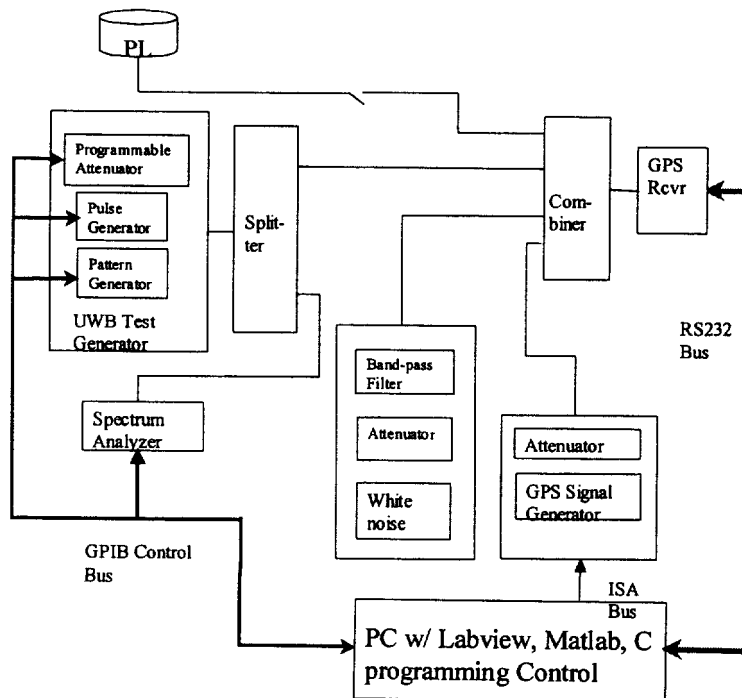
Figure 12: Full Test Setup
