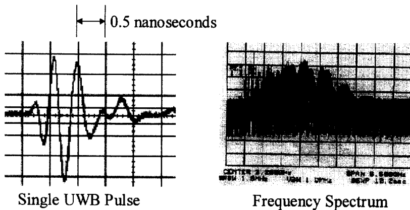
Figure 4: A UWB Signal
