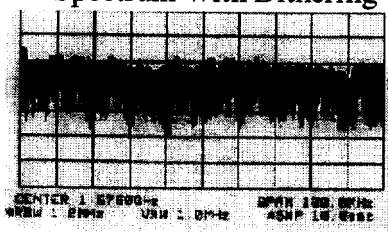
Spectrum With Dithering
