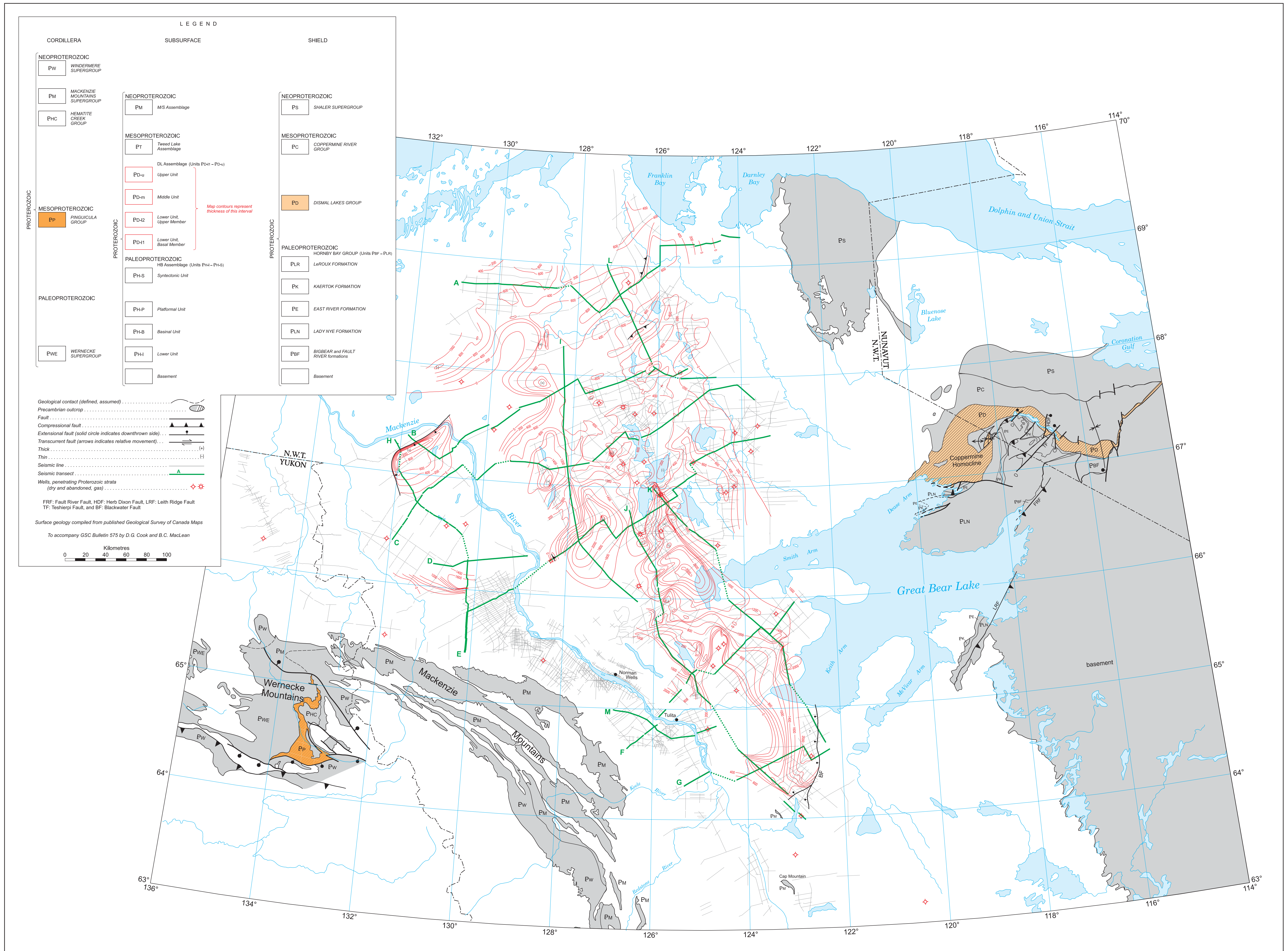
Figure 41. Seismic time-thickness map of the DL Assemblage. Contour interval is 200 ms two-way time.
