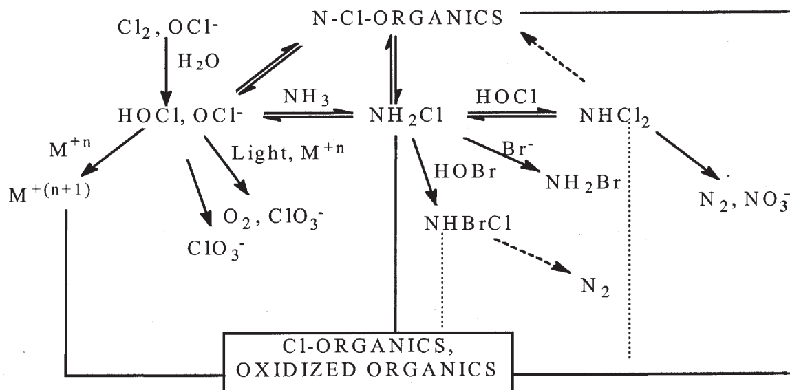
FIGURE 2 Principal chemical pathways for the reaction, degradation and fate of free chlorine in aquatic environments (adapted from Jolley and Carpenter, 1983)
