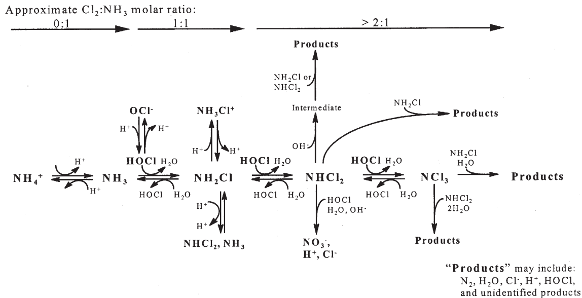
FIGURE 1 Summary of ammonia/chlorine reactions (adapted from Jafvert and Valentine, 1992)
