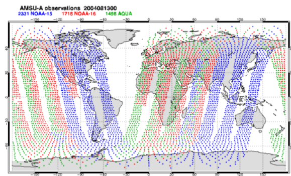
Fig. 3. An example of CMC's current AMSU-A coverage. NOAA-15 data are in blue, NOAA-16 in red and AQUA in green.
