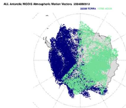
Fig. 1. Location over Antarctic of Aqua (green) and Terra (blue) SATWINDS received during the 6 hours time window centred on 12 GMT August 9, 2004.
