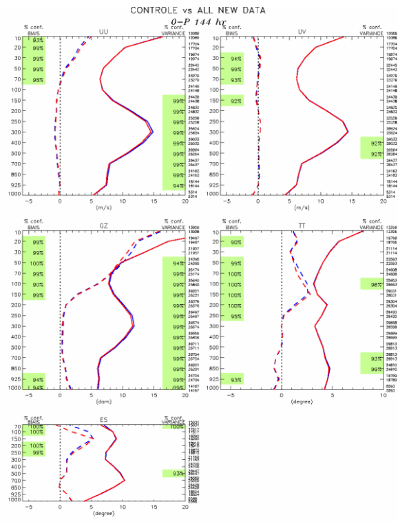
Fig. 4. Day 6 forecast root-mean-square errors (solid lines) and biases (dash lines) measured with ROABS over Northern-Hemisphere for the 123 winter 2003/04 cases. The control is in blue and the experiment is in red. The top two graphs show values for the wind components, the middle one are for the geopotential height (left) and temperature (right) and the bottom graph is for dew point departure.
