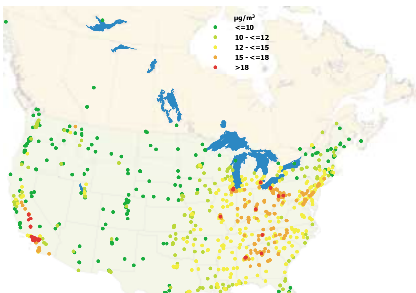
Figure 27. Mean Concentrations of PM 2.5 at Canadian Dichotomous and U.S. FRM Monitors in the Border Region (2000–2003)
