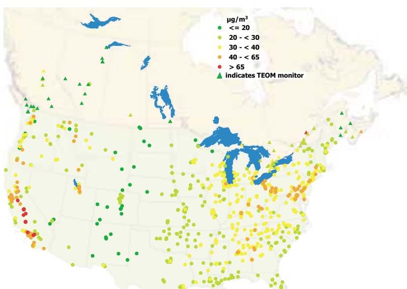
Figure 28. 98th Percentile PM 2.5 Concentrations at Canadian TEOM and U.S. FRM Sites (2000–2002)
