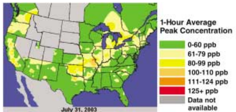
Figure 25. AIRNOW Map Illustrating Real-time Concentrations of Ground-level Ozone
