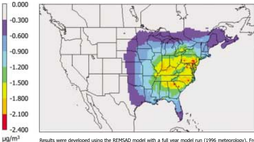
Figure 35. Anticipated Reductions in Annual PM 2.5 Concentration in 2020 from Expected U.S. and Canadian Controls
