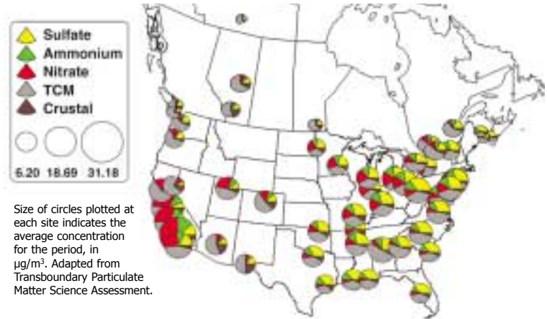
Figure 30. Summary of Rural PM_{2.5} Speciation Data from U.S. IMPROVE and Canadian Networks (September 2001–August 2002)
