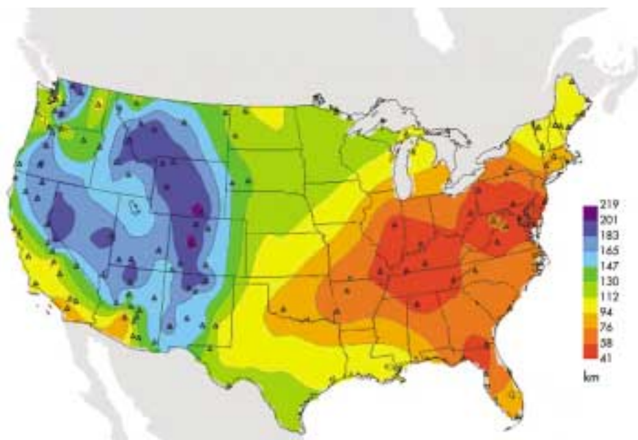
Figure 8. Annual Standard Visual Range (2002)
