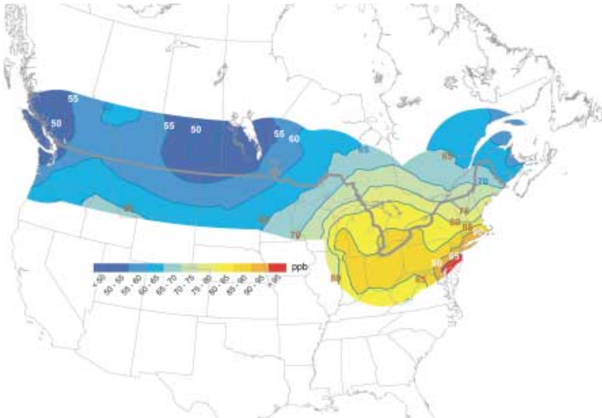
Figure 16. Ozone Concentrations (ppb) along the U.S.–Canada Border (Average Annual Fourth Highest Daily Maximum 8-Hour Average Ozone, 2000–2002)
