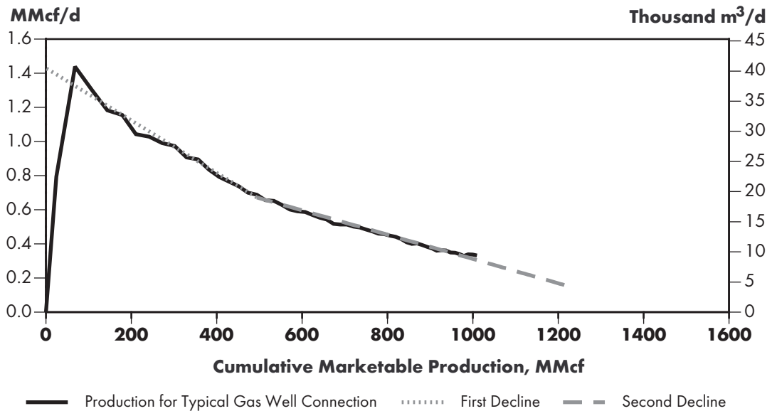
Example of Average Gas Well Connection Production Decline Plot (Alberta Foothills Front Area, 1999 Connection Year)
