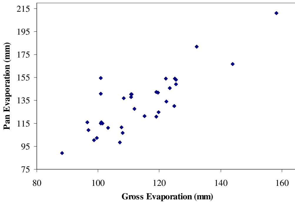
Figure D112: Scatter graph of pan evaporation vs. gross evaporation at Wynyard in September ( r = 0.83 )
