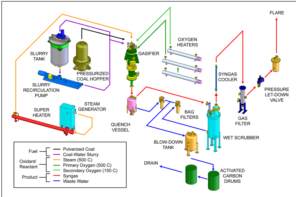
Figure 1. Flowsheet of CETC-O's Pressurized, Entrained-flow, Pilot-scale Gasification Facility
