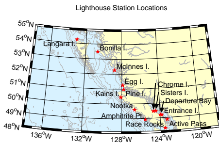
Figure 16. Lighthouse locations.
