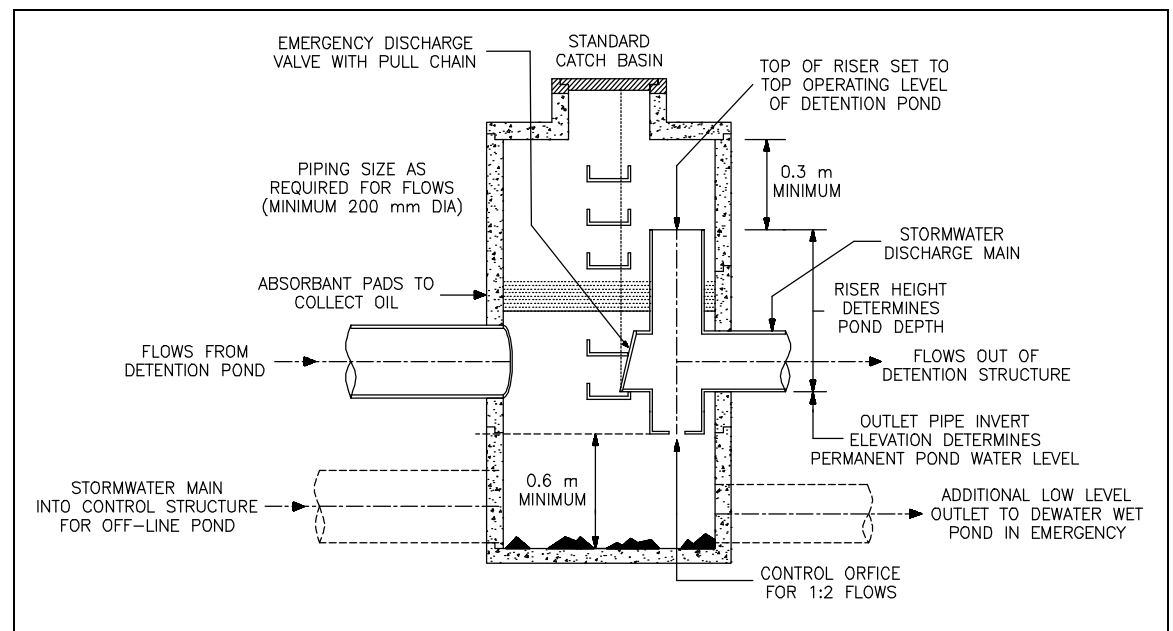
Figure 4.3 Detention Pond Control Structure Typical Details
