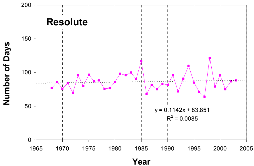
Figure 24: Number of days with air temperature above -1.8^{\circ}\text{C} at Resolute throughout period of 1968-2003
