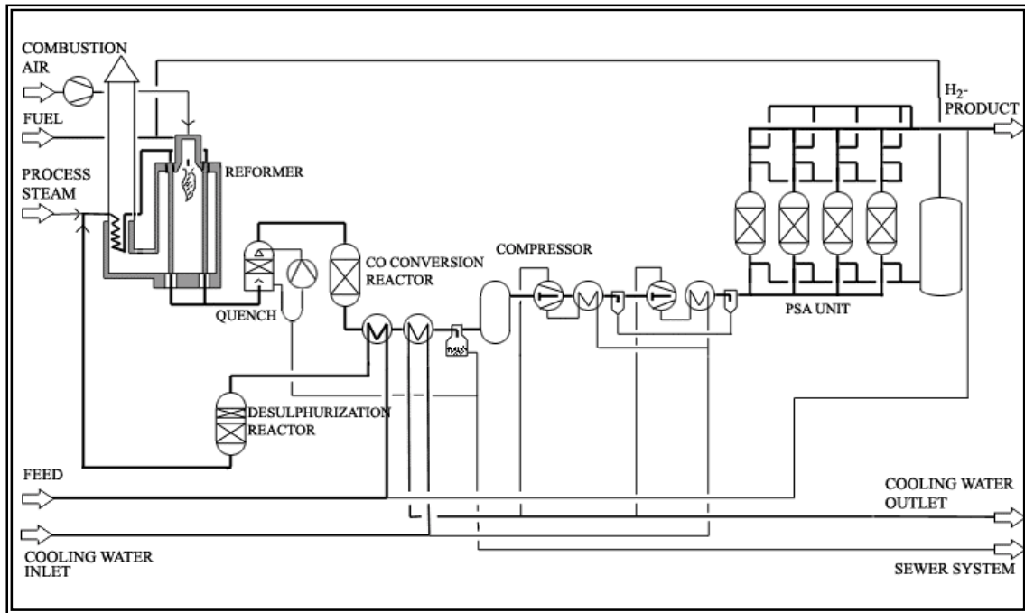
Figure 2-2 LPG Reforming
