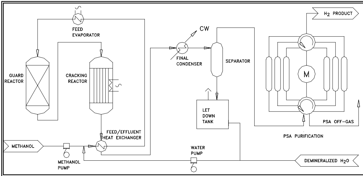
Figure 2-1 Methanol to Hydrogen Reformers
