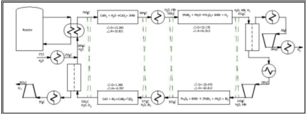
Figure 2-4 UT-3 Flow Diagram
