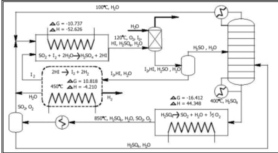
Figure 2-5 Sulphur-Iodine Cycle
