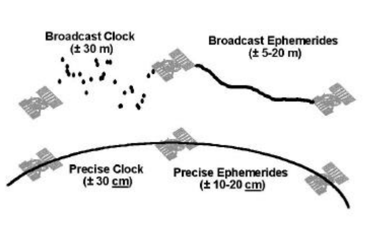
Figure 3: Satellite data improvements resulting from Canadian Active Control System (CACS) processing [1]
