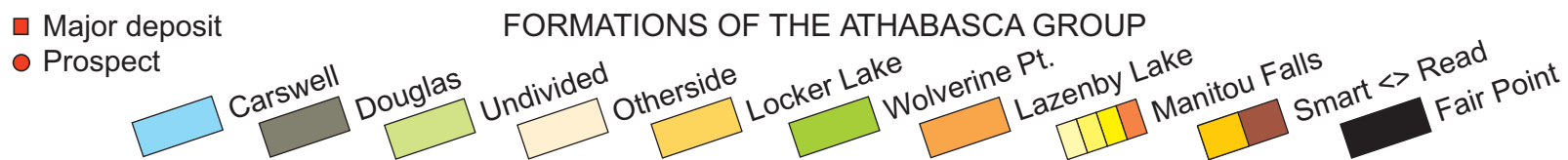
Some Uranium Occurrences in the Athabasca Basin, Northern Saskatchewan and Alberta.
