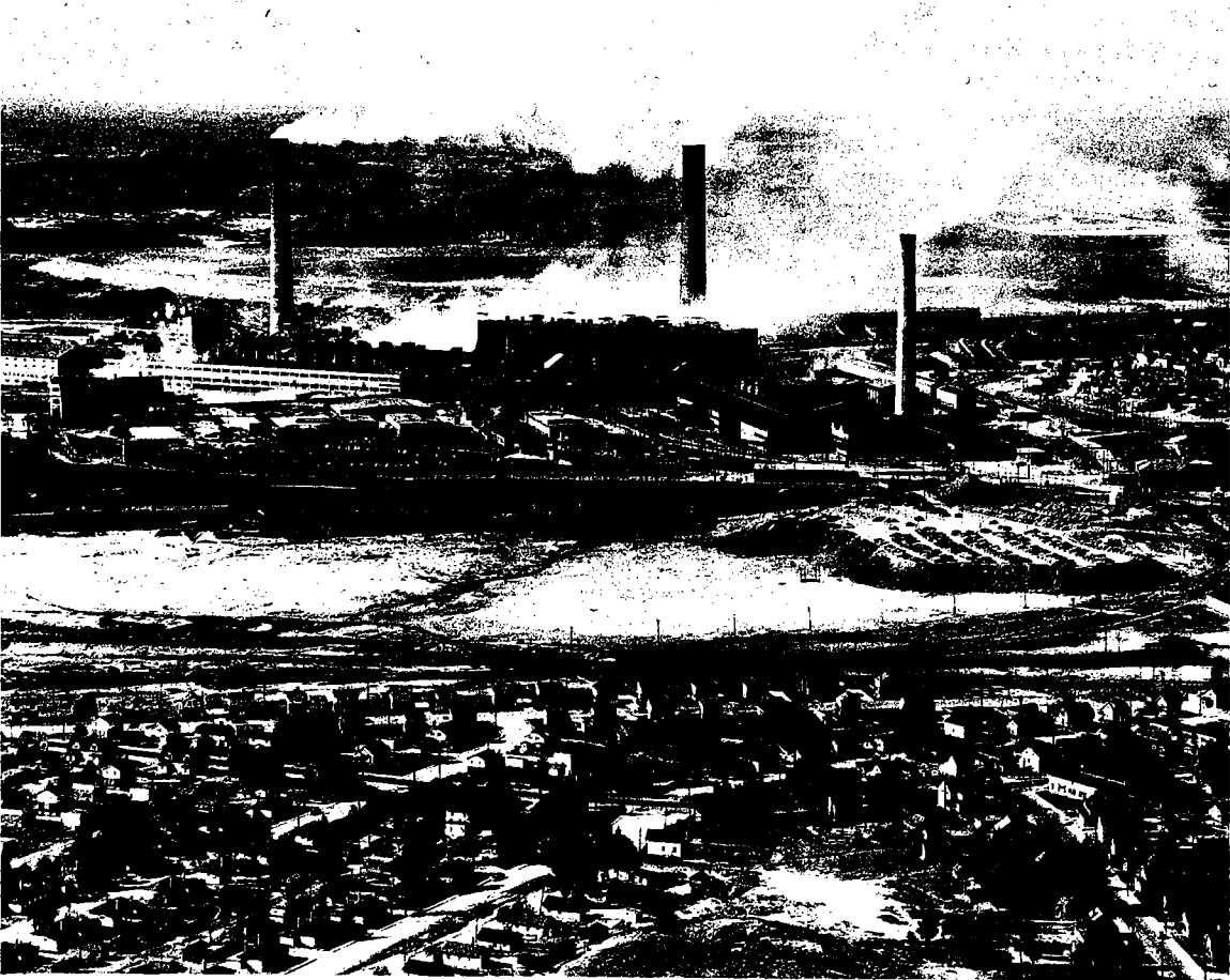
Located at Copper Cliff, Ontario, International Nickel Company's mill has a capacity of 30,000 tons of ore a day. The smelter has seven reverberatory furnaces and nineteen converters.
