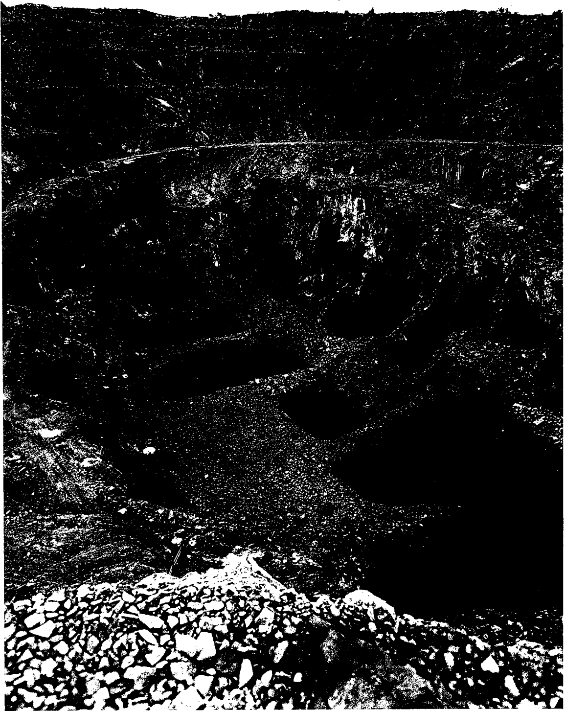
Blast-hole stopes surfacing at the bottom of the Froid-Stobie open pit. Scale is indicated by the drill rigs at the upper left.
