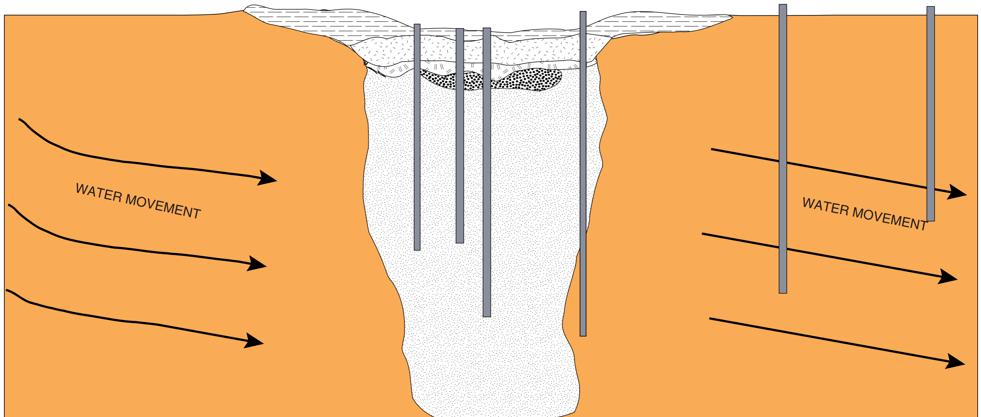
Figure = conceptual model of groundwater interaction with kimberlites.
