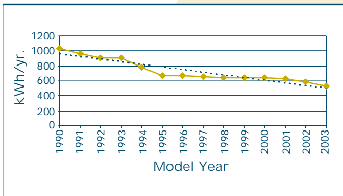
FIGURE 3.3 Average Annual Unit Energy Consumption of Dishwashers by Model Year*
