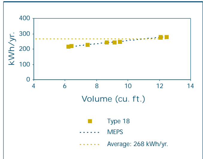
Energy Consumption of Type 18 Freezer Models Available in 2003
