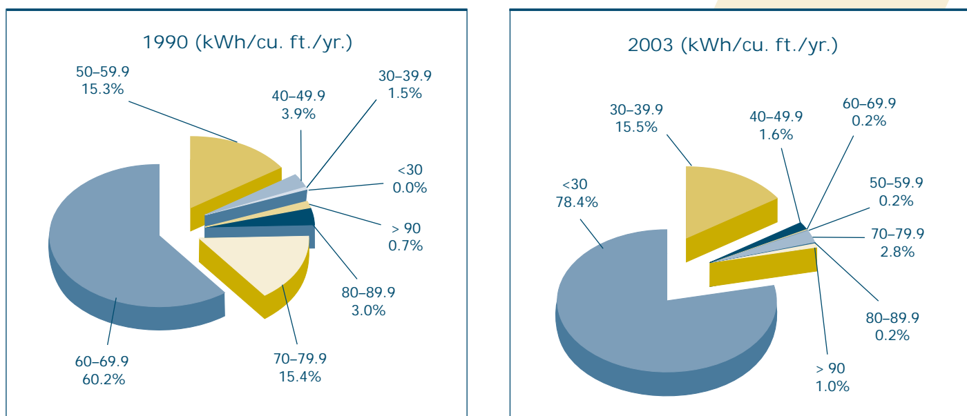
Distribution of Refrigerators by Average Annual Unit Energy Consumption per Cubic Foot for 1990 and 2003
