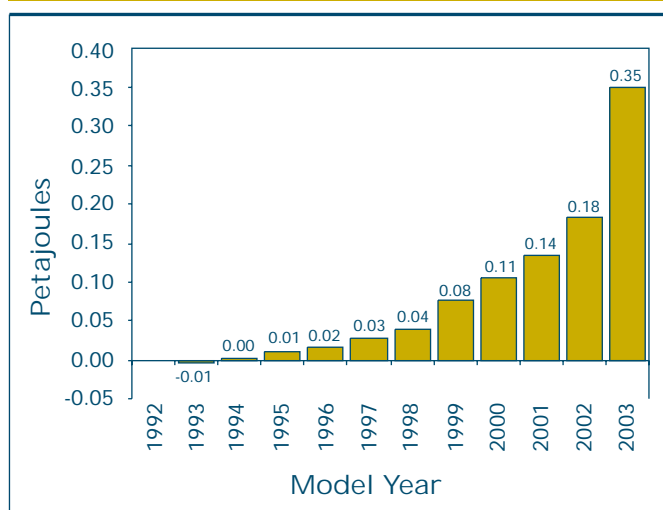
FIGURE 4.6 Cumulative Energy Savings for Electric Ranges, 1992–2003*
