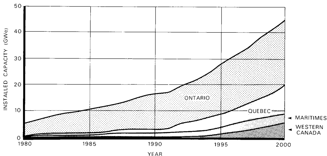
NUCLEAR CAPACITY IN CANADA FORECAST TO 2000
