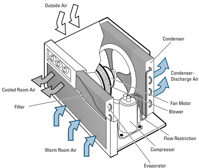
Figure 3 Components of a room air conditioner
