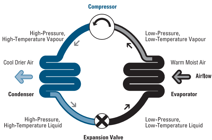
Figure 4 Basic cooling cycle
