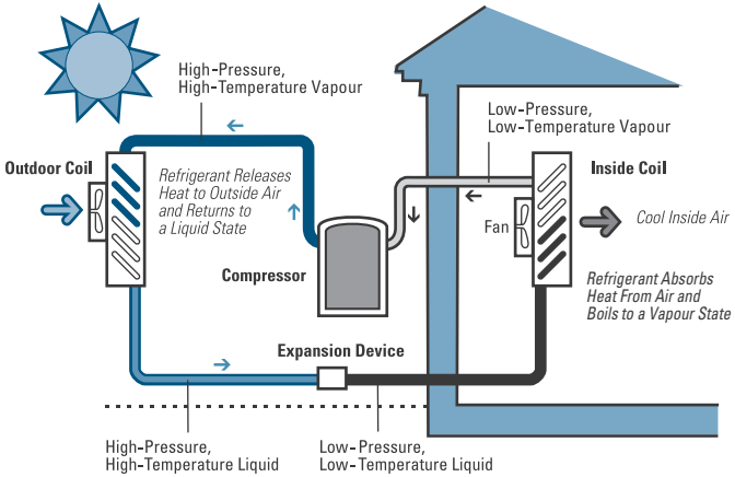
Figure 7 The operation of a central air conditioner
