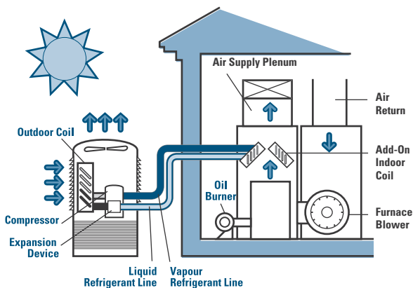
Figure 6 Installed central air conditioner
