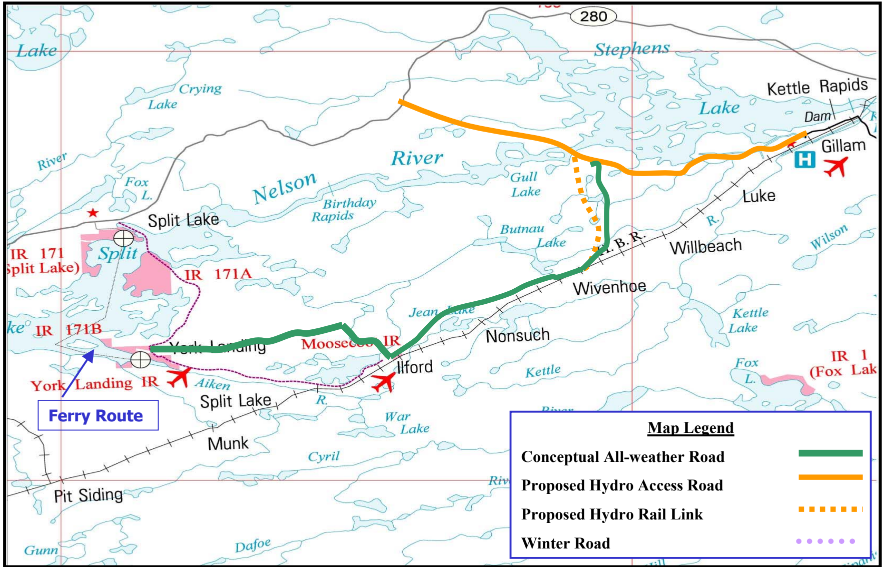
ILFORD CONCEPTUAL ALL-WEATHER ROAD - OPTION 2 FIGURE 3
