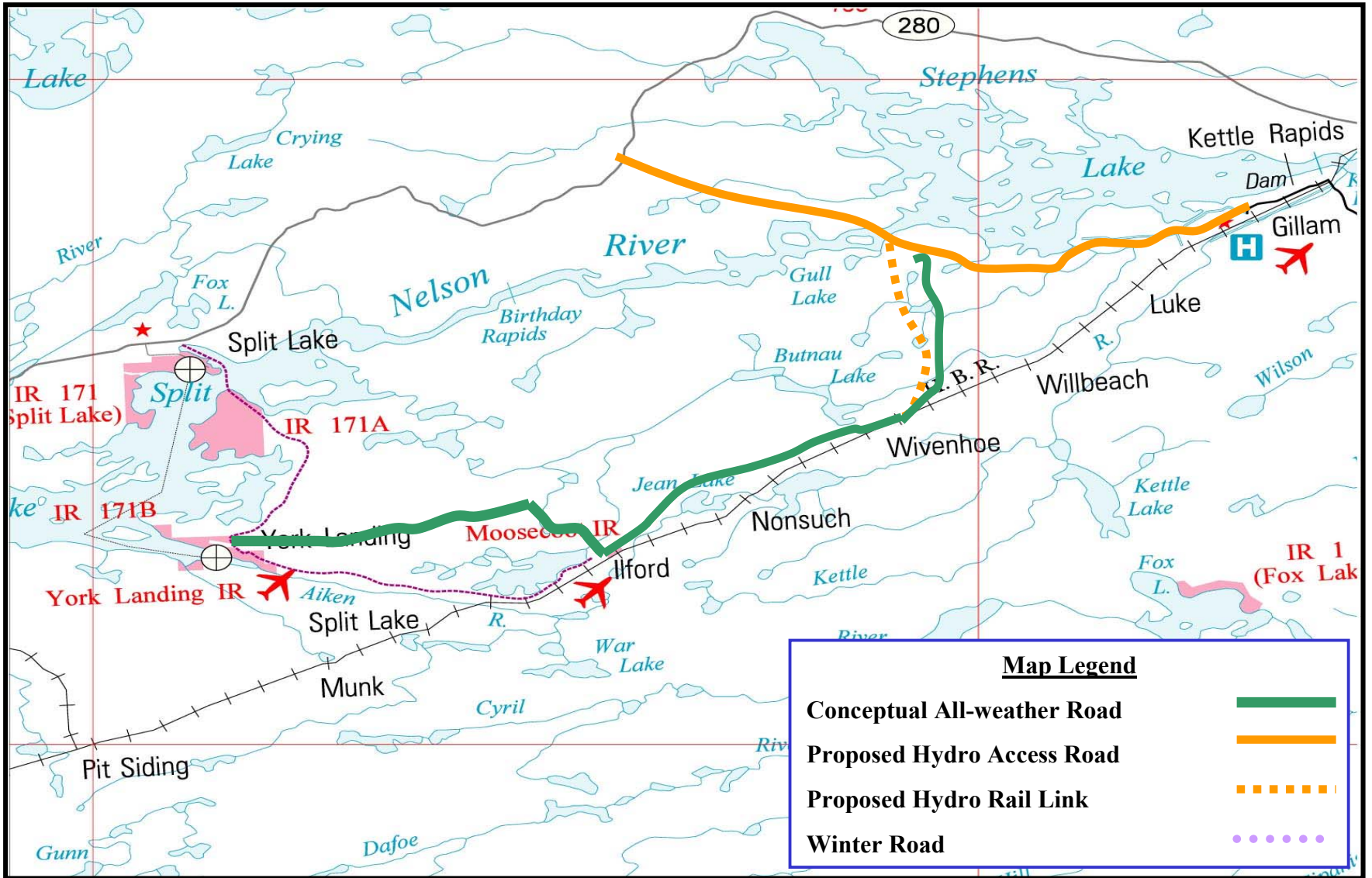
YORK LANDING – ILFORD, CONCEPTUAL ALL WEATHER ROAD VIA THE PROPOSED GULL LAKE HYDRO ELECTRIC DAM - OPTION 2 FIGURE 3
