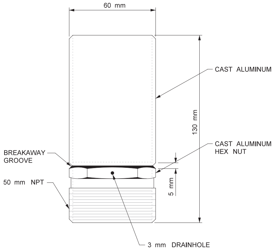
ELEVATION VIEW SAT - 9300 - 4M T/C TYPE 1
