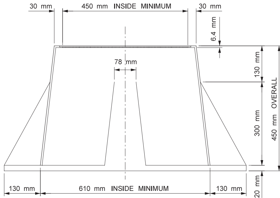
ELEVATION VIEW
