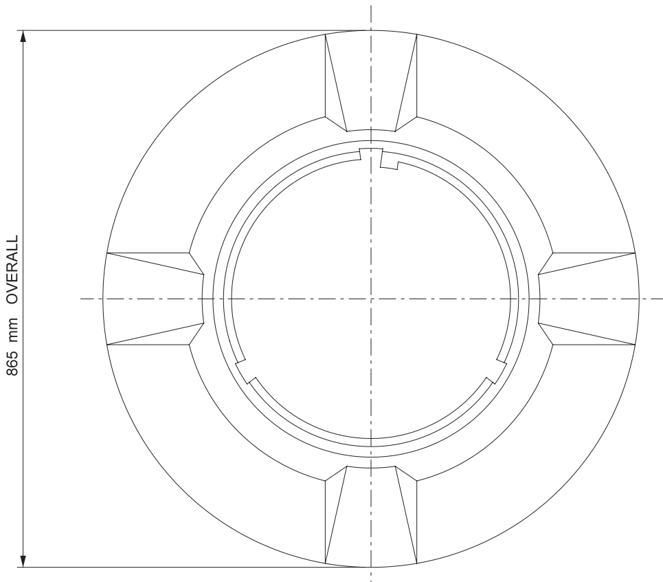
PLAN VIEW
