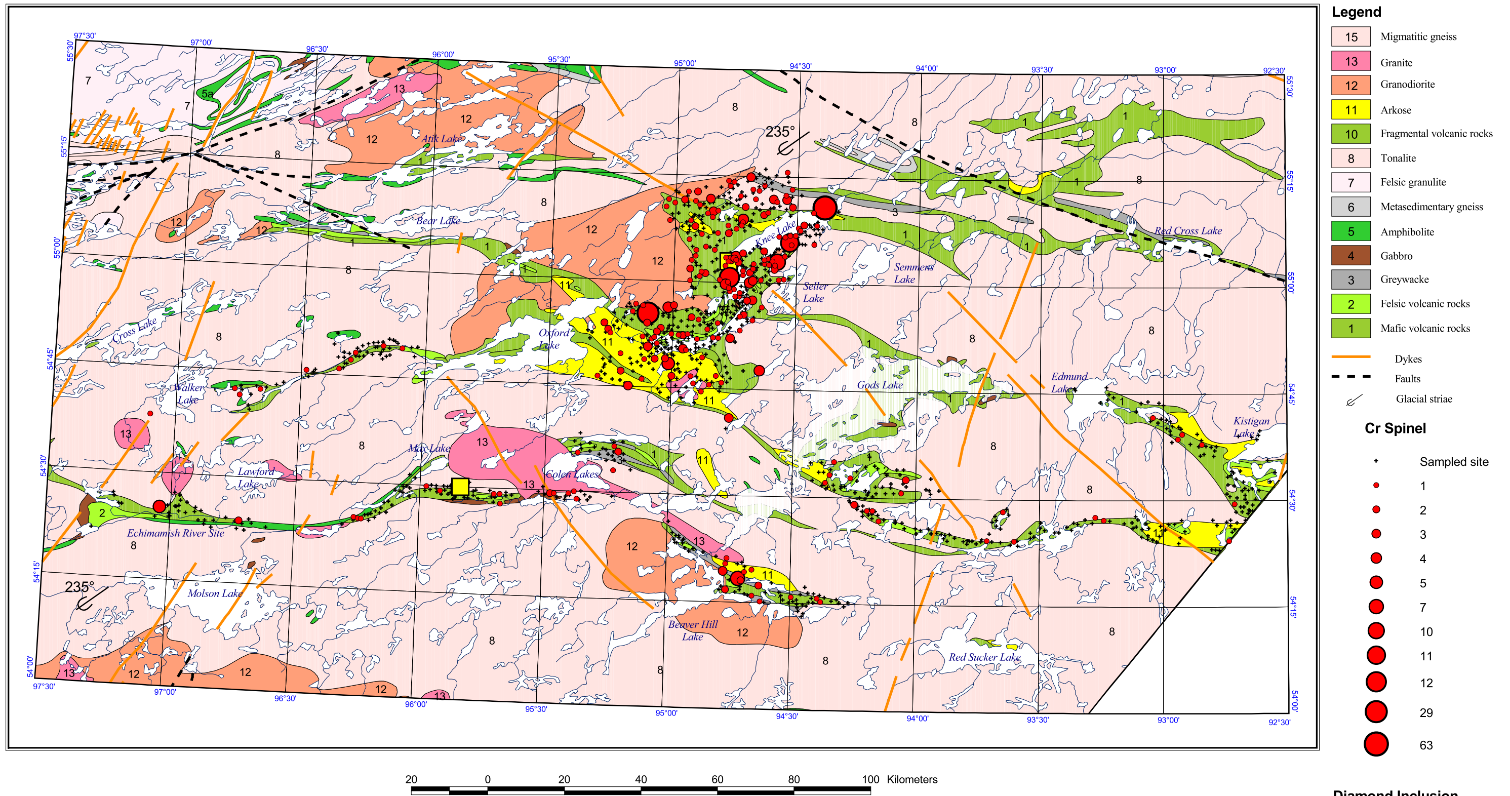
Figure 2. Regional distribution of Cr-spinel grains, Operation Superior, 1996-2000.
