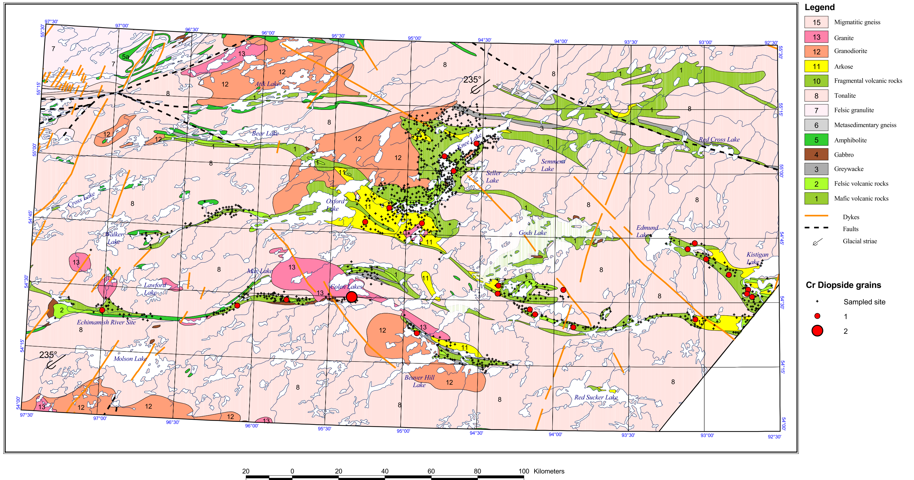
Figure 3. Regional distribution of Cr-diopside grains, Operation Superior, 1996-2000.
