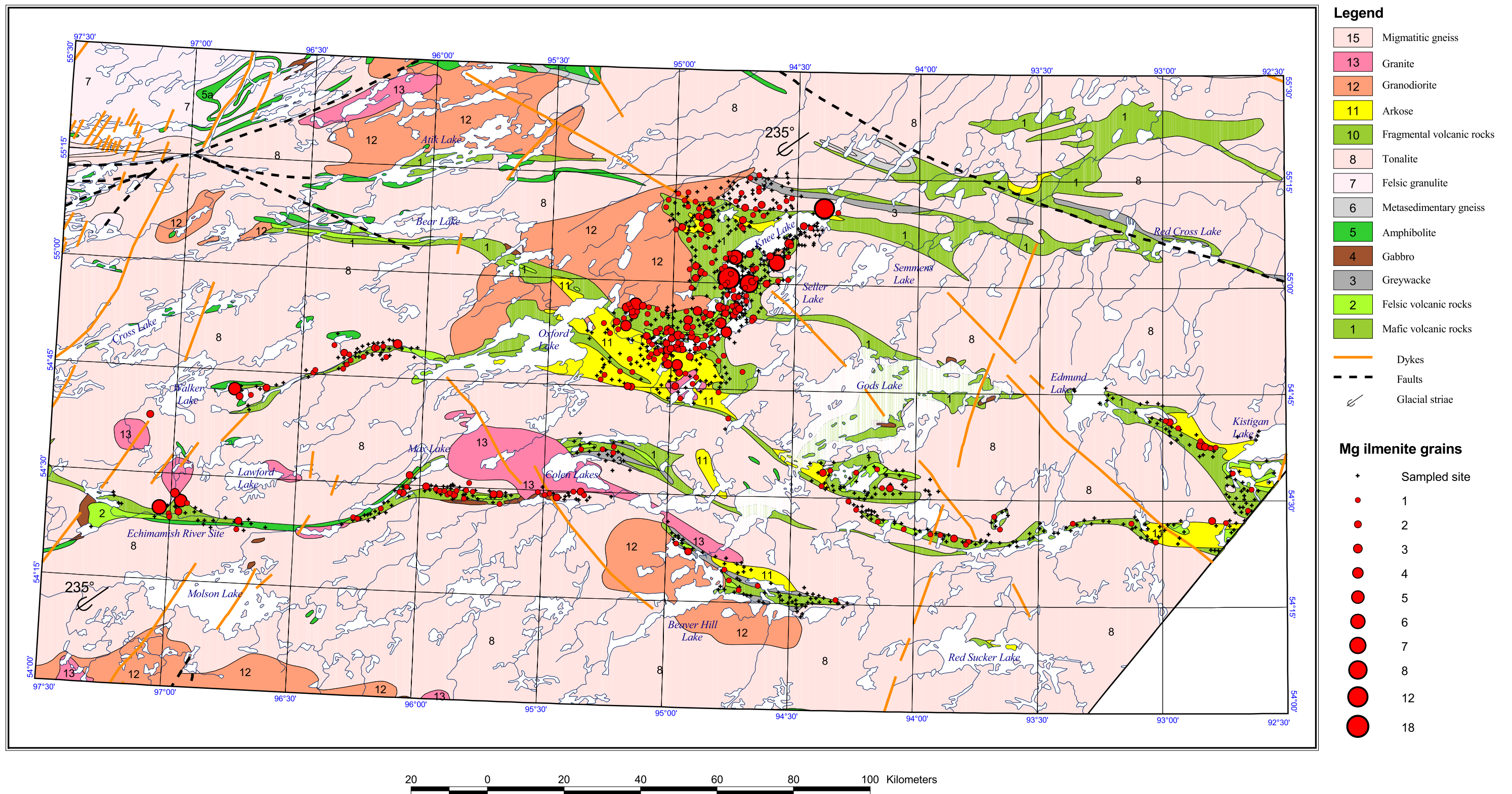
Figure 7. Regional distribution of Mg-ilmenite grains, Operation Superior, 1996-2000.
