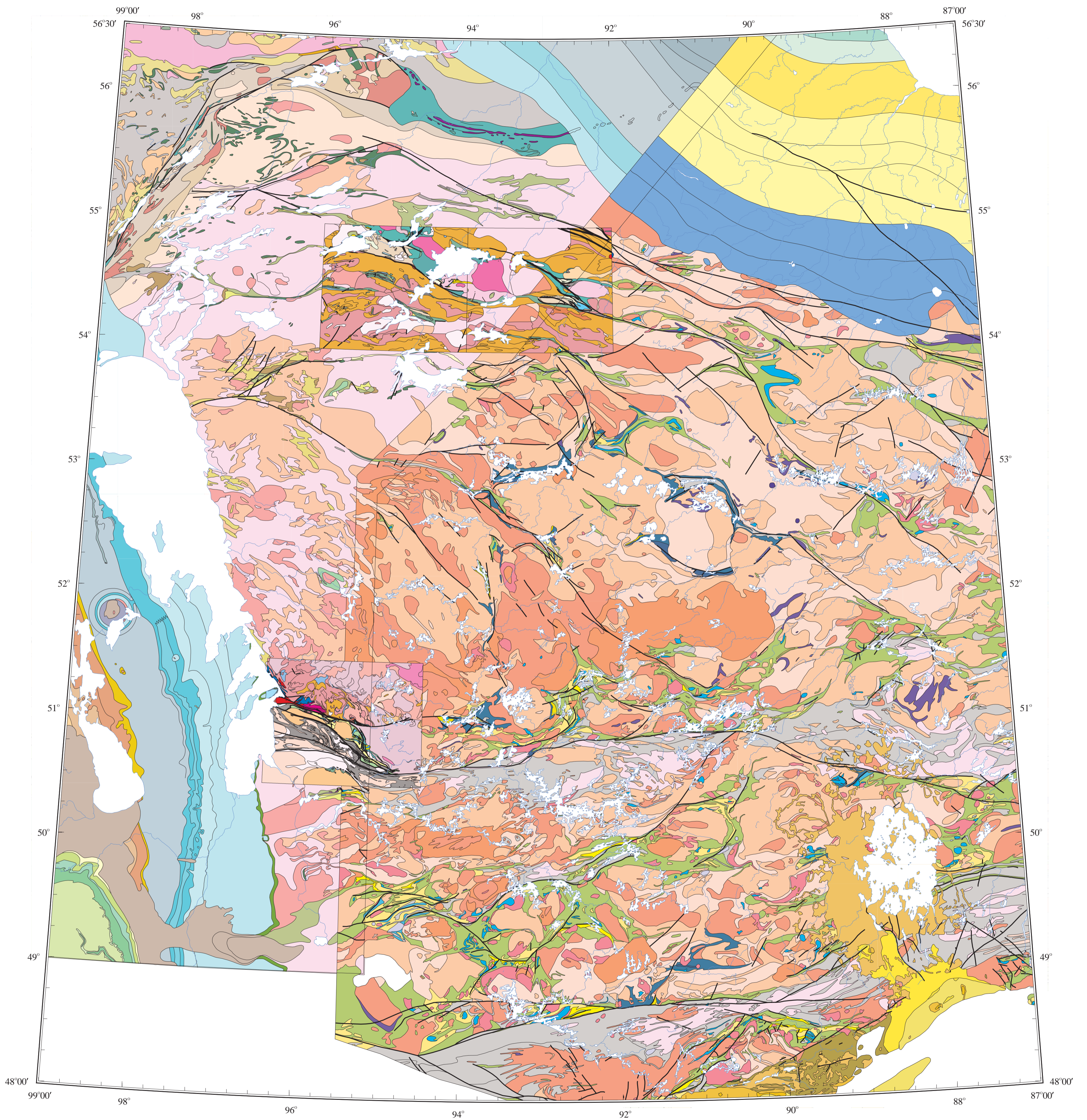
Figure 9. Western Superior NATMAP 1:2 000 000 scale geologic map of the Superior Province. Insert maps covering the areas of 1:250 000 scale compilation maps are shown, generally in darker colours, for the Oxford and Stull lakes area in northern Superior Province as well as for the Bissett area in southeast Manitoba.
