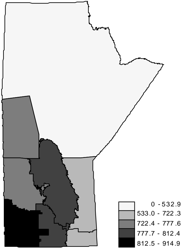
All sites (ICD-9 140-208, 230-239) - Males Incidence Rates (per 100,000) 1990-96
