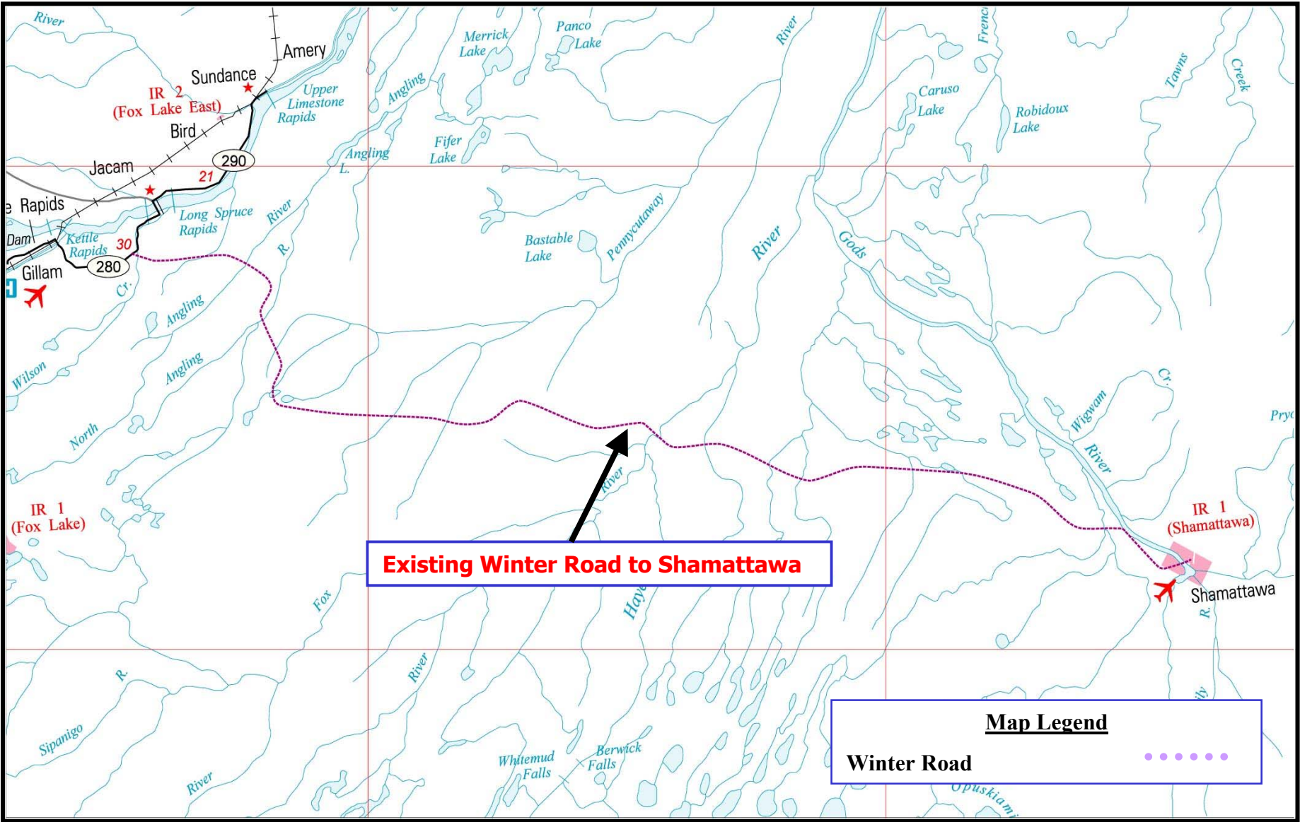
SHAMATTAWA AREA – WINTER ROAD SITE LOCATION PLAN FIGURE 1
