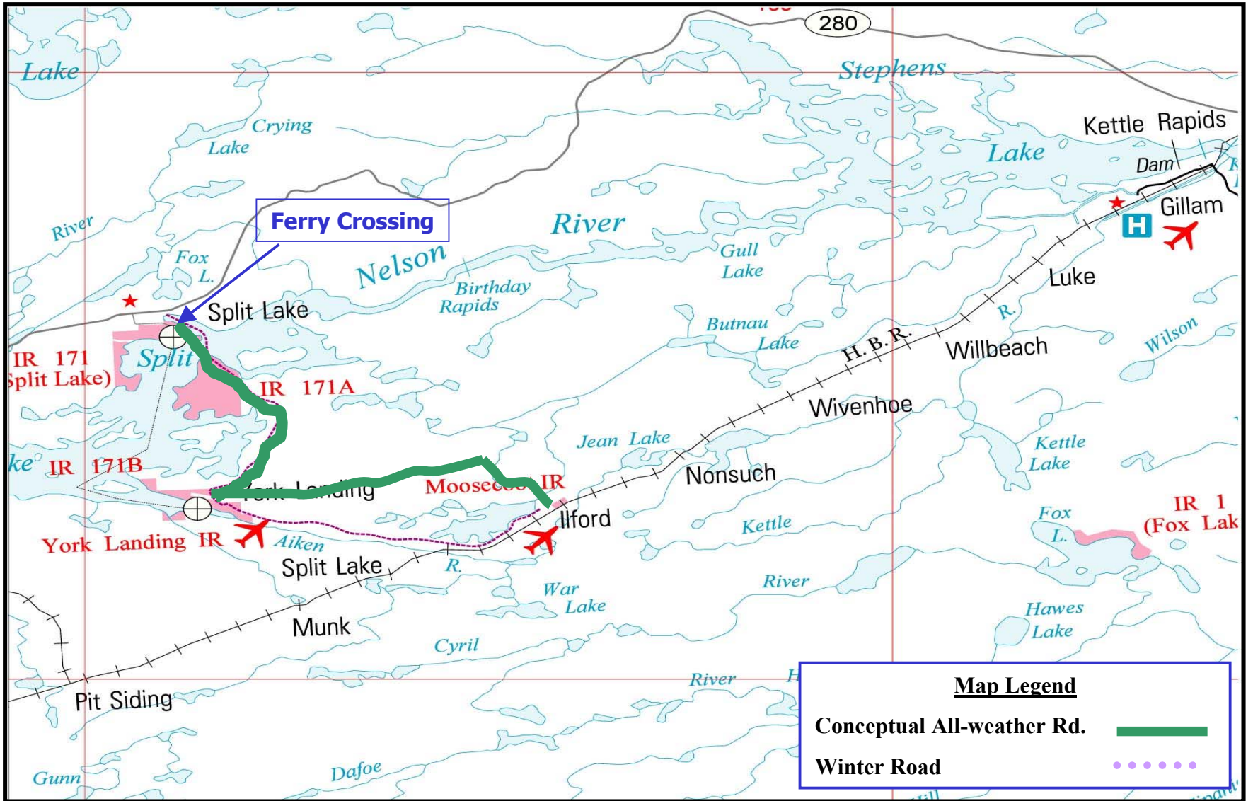
YORK LANDING –ILFORD, CONCEPTUAL ALL WEATHER ROAD AROUND SPLIT LAKE AND FERRY CROSSING - OPTION 5 FIGURE 6
