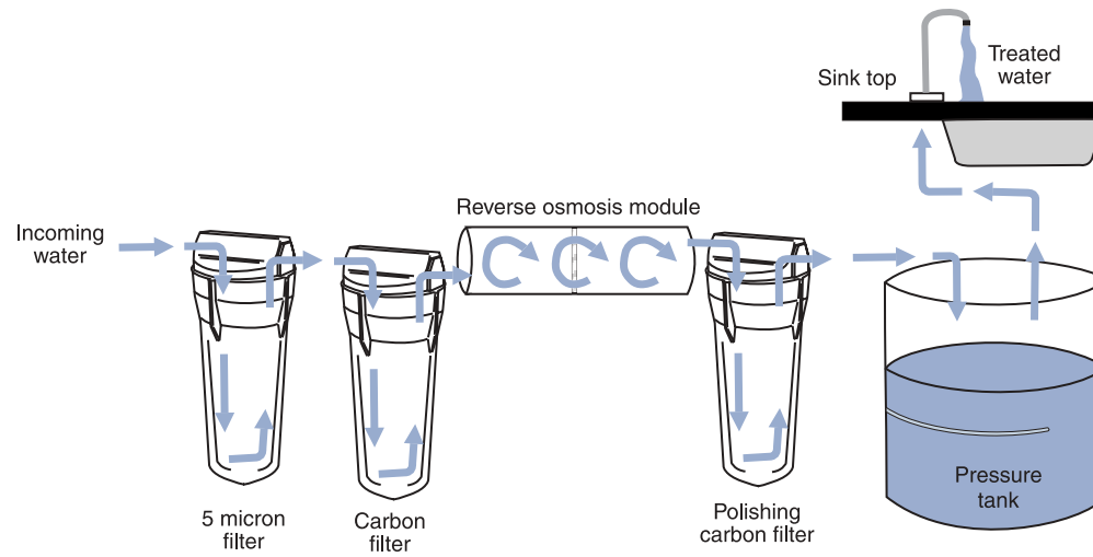
Figure 41 RO Treatment Process
