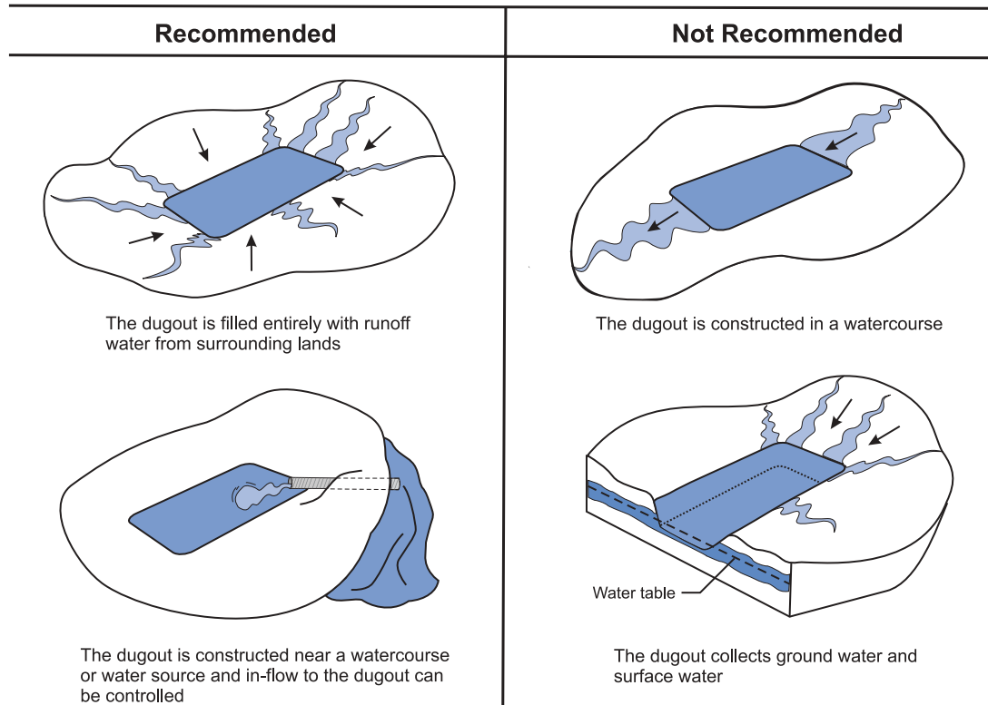
Figure 3 Dugout Types
