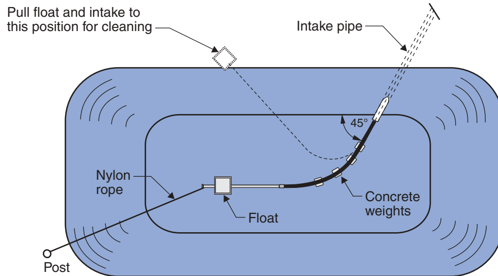
Figure 25 Plan View of Intake System
