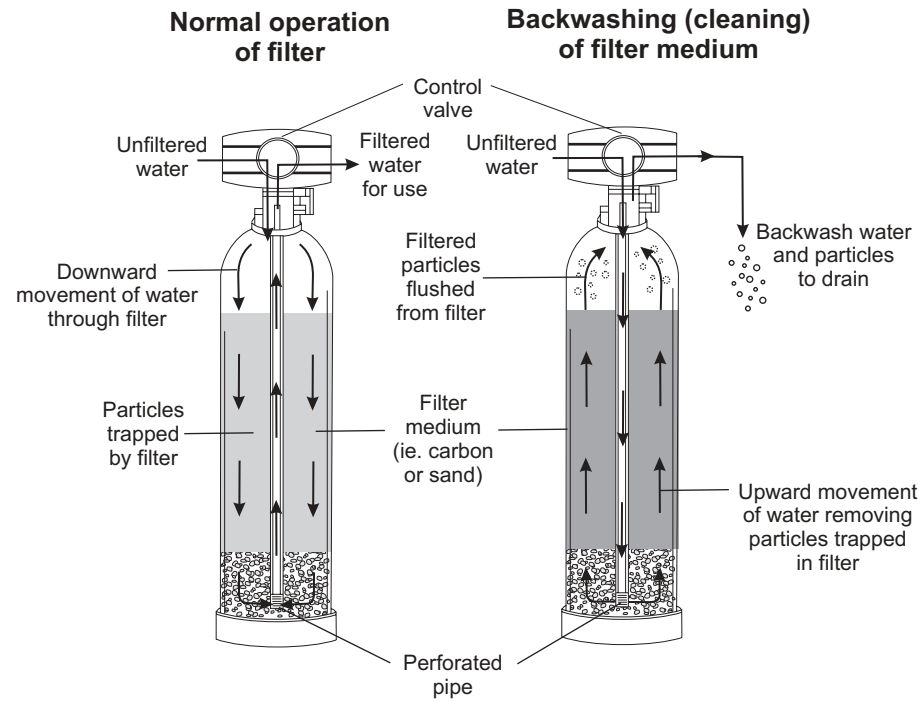
Figure 39 Filter Backwashing
