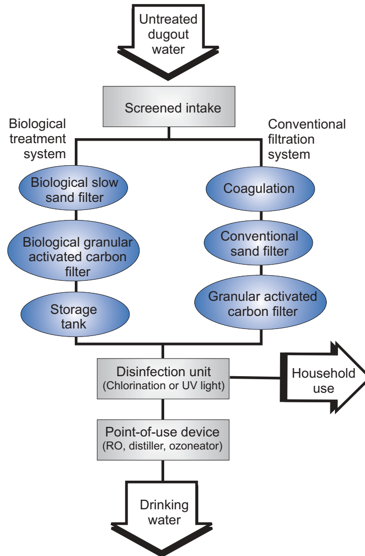
Figure 36 Surface Water Treatment Steps
