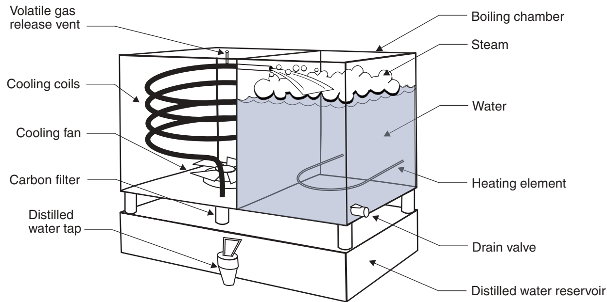
Figure 40 Water Distiller
