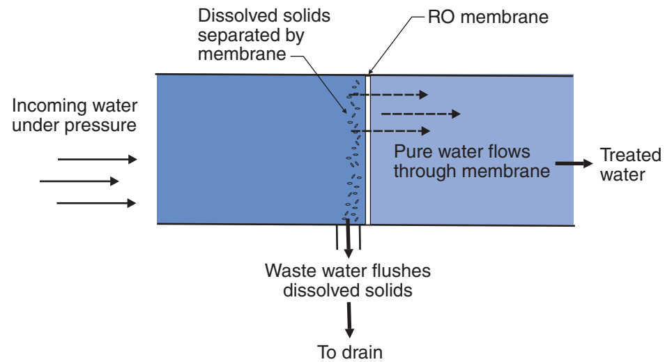
Figure 42 RO Membrane
