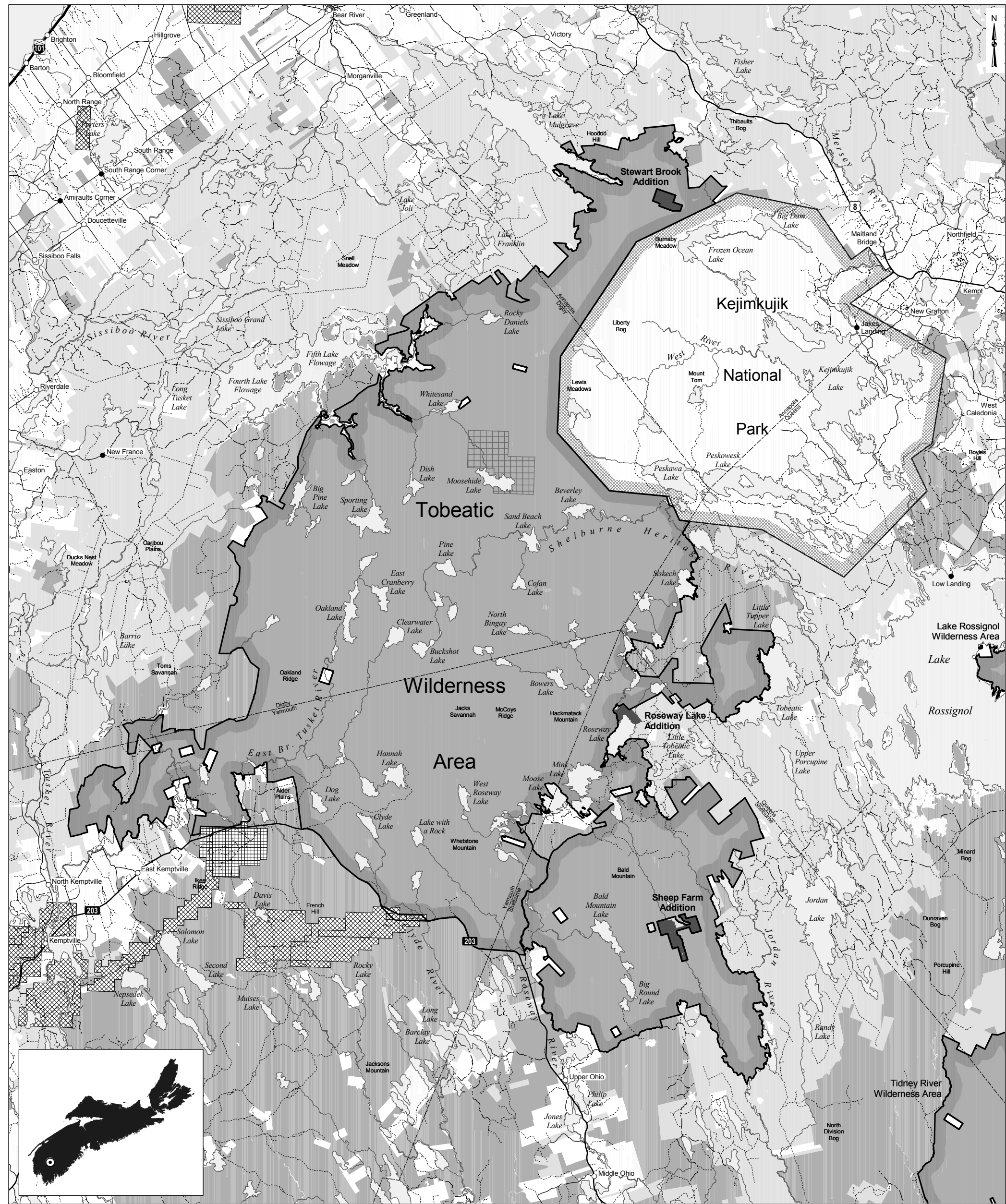
Figure 6. Tobeatic Wilderness Area - Adjacent Ownership & Land Use
