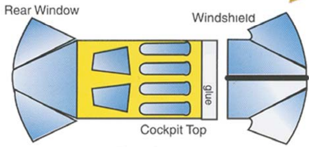
Fuselage
