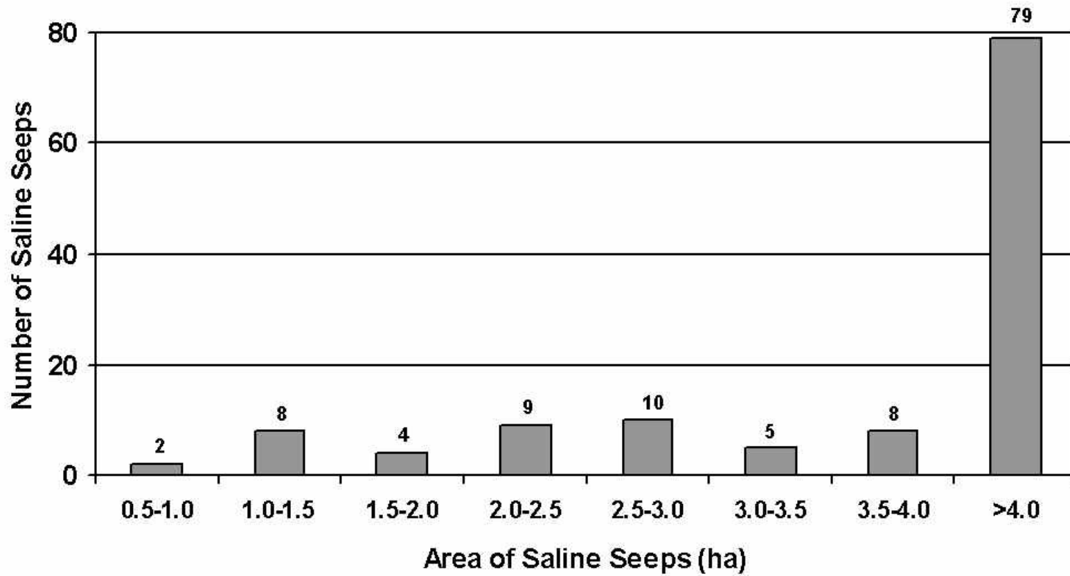
Figure 10. Number and Size of Total Saline Seeps in the M.D. of Acadia
