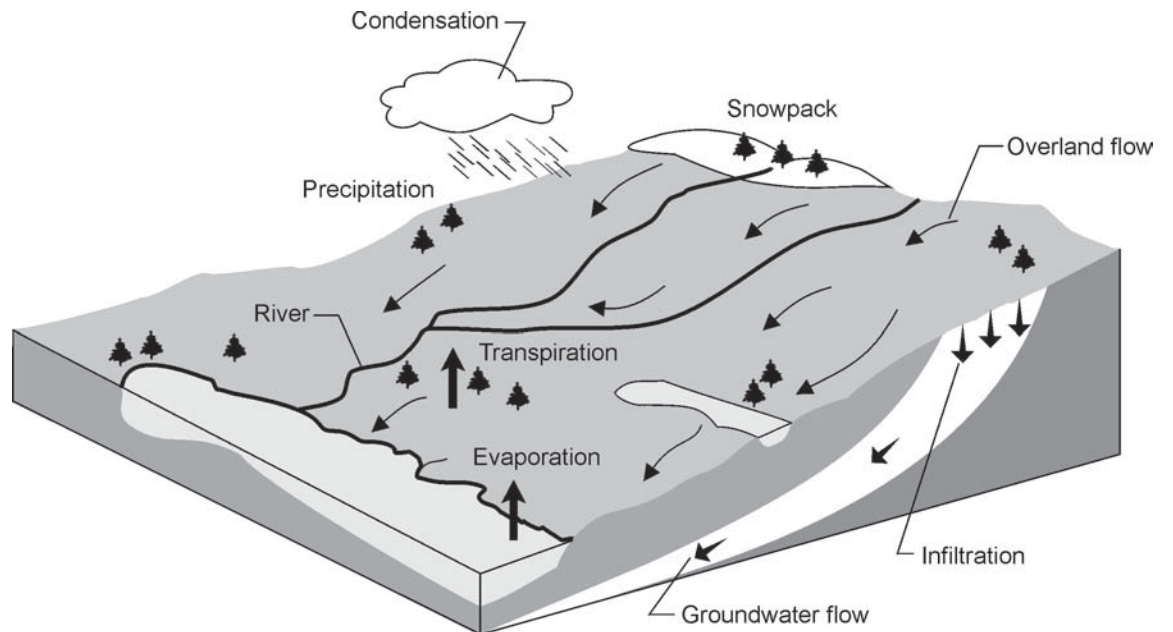
Figure 1 Hydrologic Cycle
