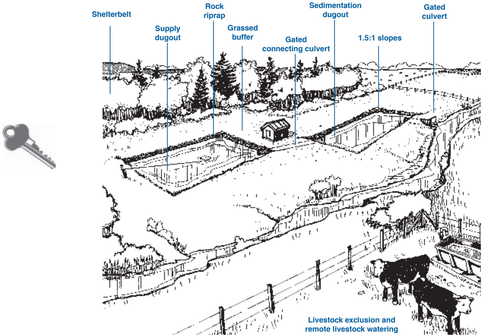
Figure 16 Dugout with Design Best Management Practices
