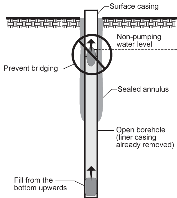
Figure 3 Bridging
