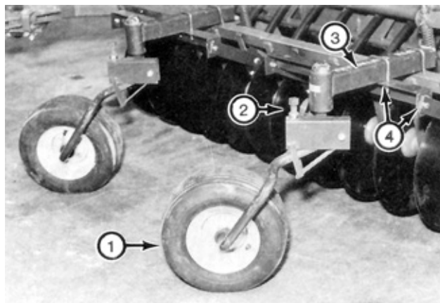
FIGURE 1. Jeannotte Controller Mounted to Disk Gang (1) Castoring Wheel, (2) Depth Adjustment Screw, (3) Mounting Arm, (4) Mounting Brackets and Clamps.
