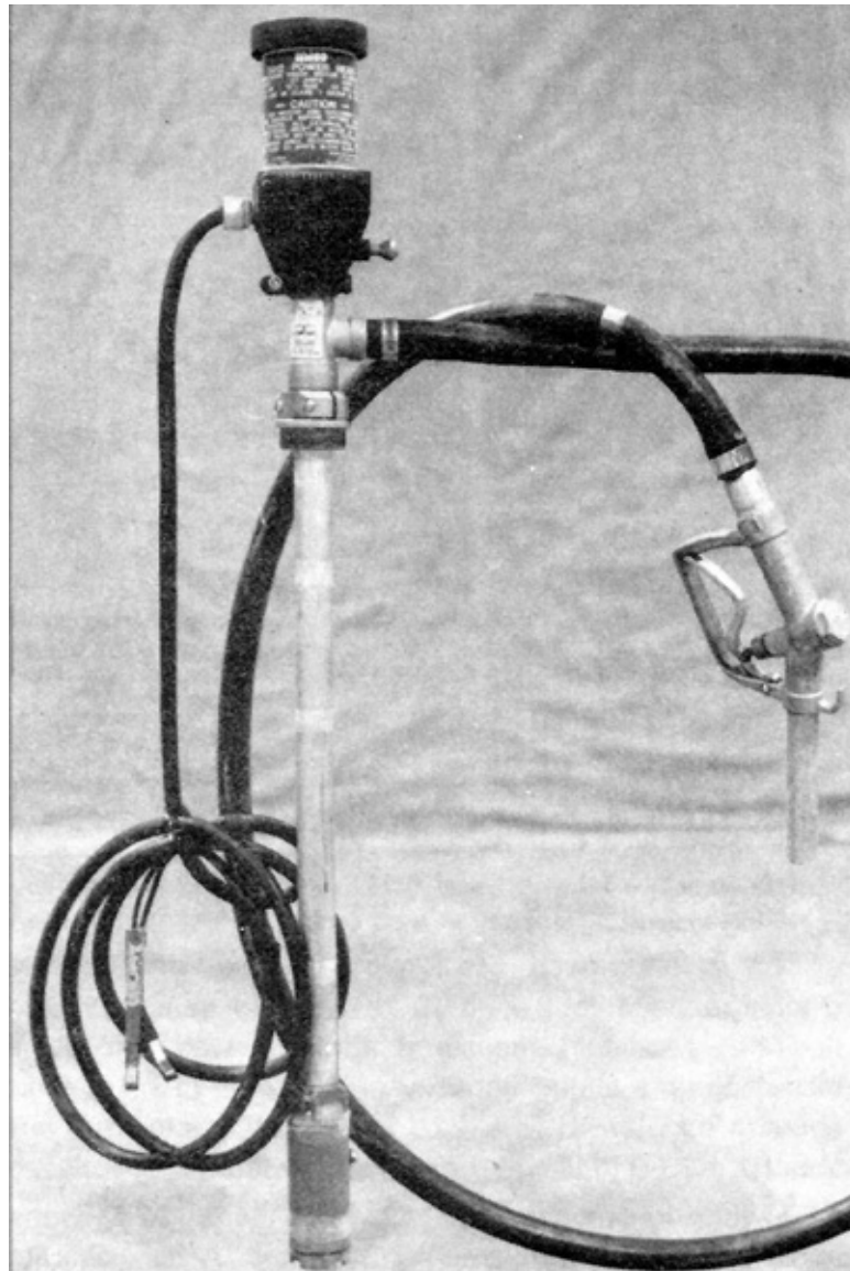
Mico 5012 Series (Model 02-820-012) Fuel Transfer Pump
