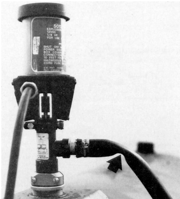
FIGURE 5. Kinked Outlet Hose.
