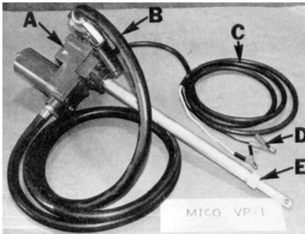
FIGURE 1. Mico Model VP-1 Fuel Transfer Pump: (A) Pump Body, (B) Outlet Hose, (C) Battery Cable, (D) Battery Clamps, (E) Telescoping Suction Pipe.
