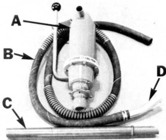
FIGURE 1. Macnaught Litre-Stroke Hand Pump: (A) Pump Body, (B) Outlet Hose, (C) Telescopic Suction Pipe, (D) Outlet Nozzle.
