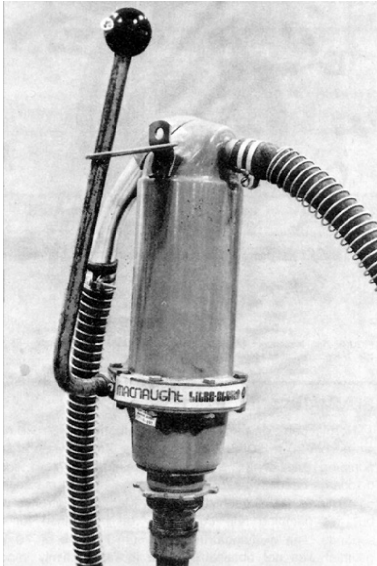
Macnaught Litre-Stroke Hand Pump
