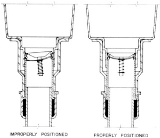
FIGURE 5. Inlet Valve Assembly.
