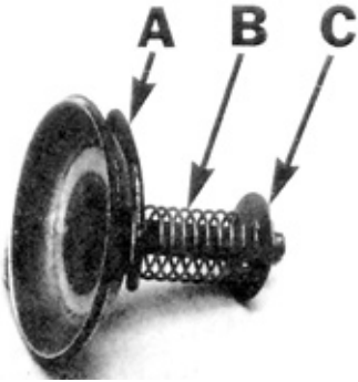
FIGURE 4. Inlet Valve Assembly: (A) Circlip, (B) Spring, (C) Ratchet Plate.
