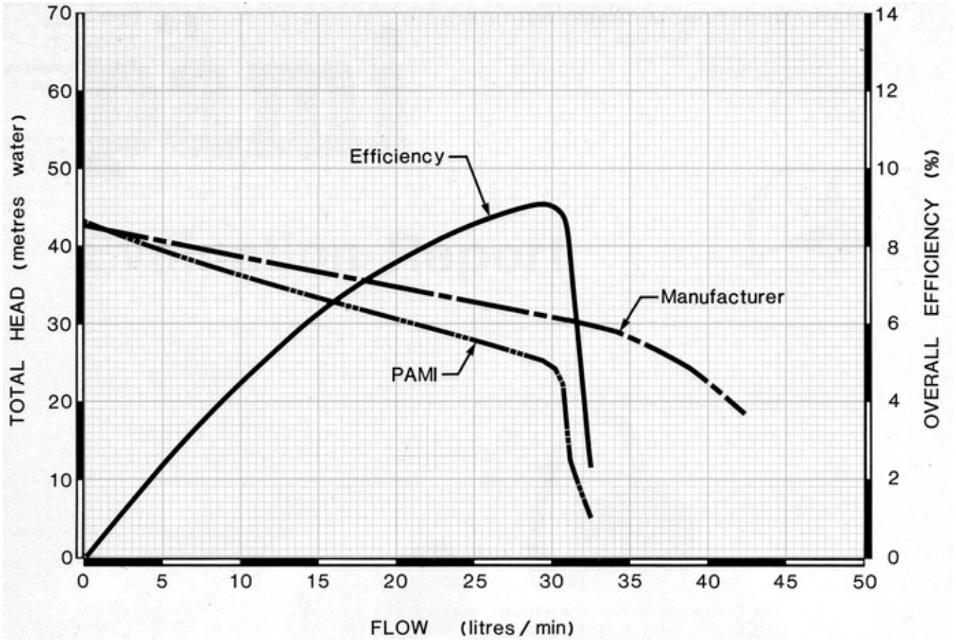
FIGURE 1. Performance Characteristics.
