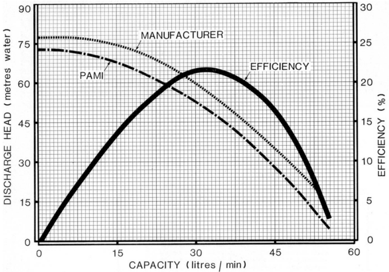
FIGURE 1. Performance Characteristics.
