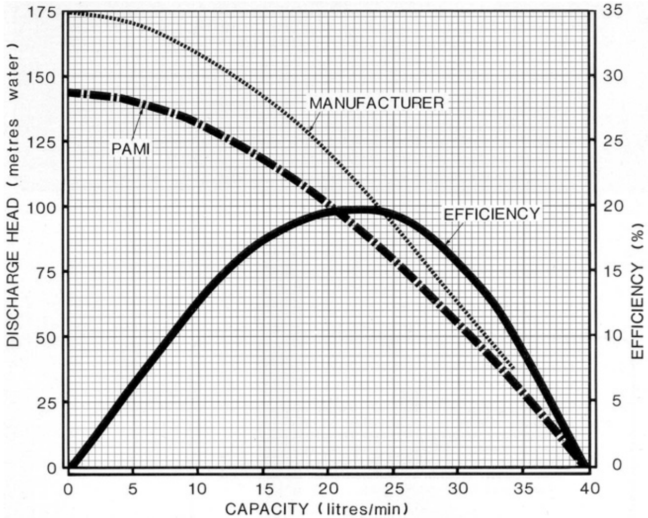
FIGURE 1. Performance Characteristics
