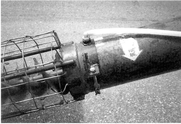
FIGURE 6. Liquid Outlet into Grain Stream.
