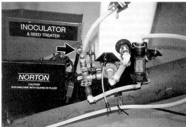
FIGURE 7. Interference Between Hopper and Return Line when Adjusting for Steep Auger Angles.
