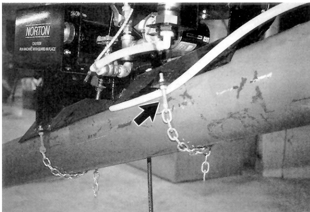
FIGURE 8. Restricted liquid line when Fastened Behind Clamps.
