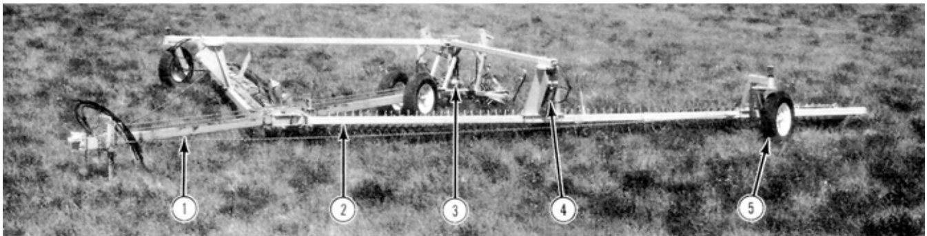
FIGURE 1. Phoenix Rotary Harrow Model HT140: 1) Hitch Frame, 2) Wing Frame, 3) Transport Motor Drive Location, 4) Tine Lift Cylinders, 5) Wing Wheels.
