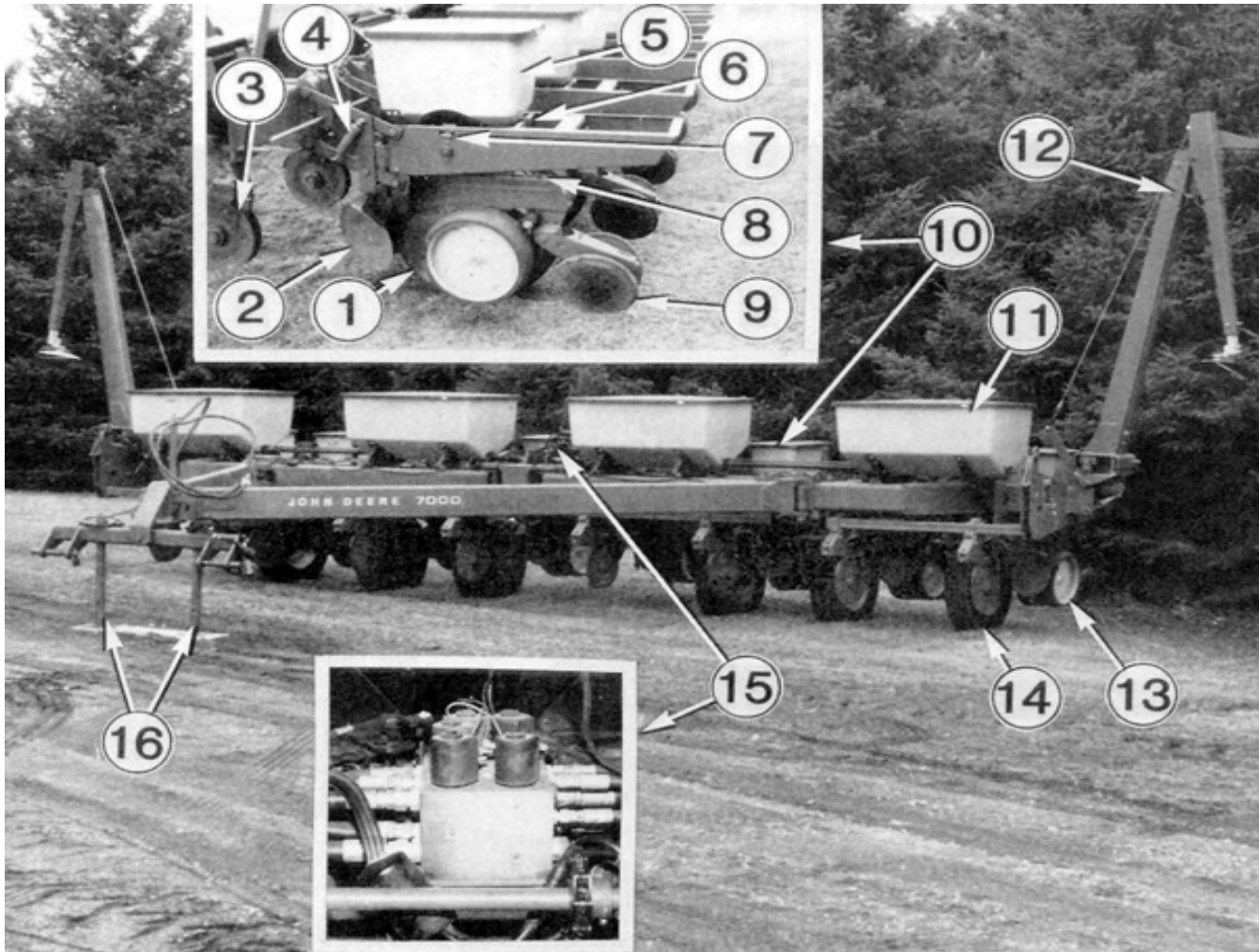
FIGURE 1. John Deere 70(X) Max-Emerge: (1) Seed Disk Openers, (2) Disk Furrowers, (3) Fertilizer Disk Openers, (4) Down Pressure Springs, (5) Seed Hopper, (6) Seed Hopper Latch, (7) Seed Drive Release Mechanism, (8) Depth Control Adjustment, (9) Closing Wheels, (10) Seed Unit, (11) Granular Fertilizer Hoppers, (12) Hydraulic Row Markers, (13) Depth Gauge Wheels, (14) Ground Wheels, (15) Solenoids, (16) Safety Stands.
