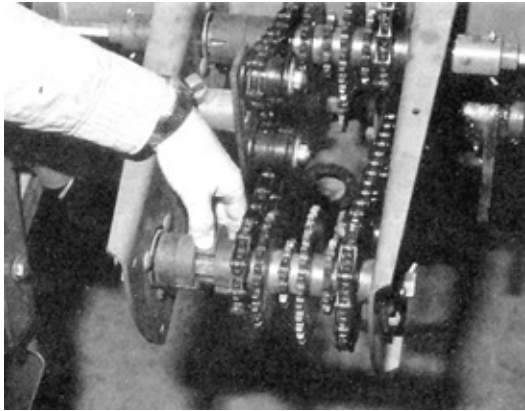
FIGURE 4. Seed Drive Transmission.
