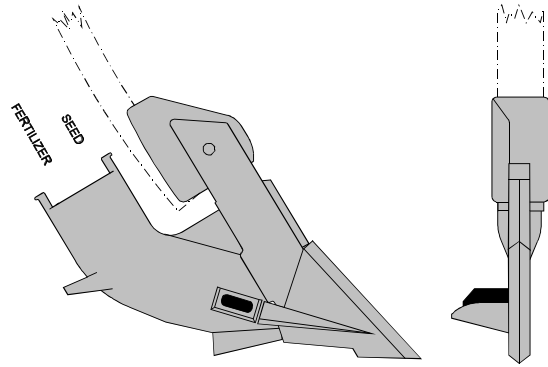
Figure 1. GEN 200 T2 Seeding System.
