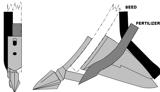
Figure 1. Dutch Vern Eaglebuster Combination.
