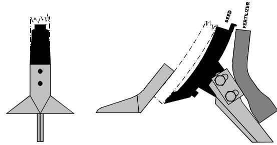
Figure 1. Key Ag Seven Inch Chrome With Backswept Knife.
