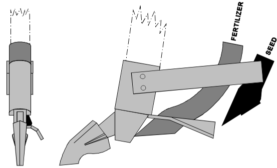
Figure 1. Morris Edge-on Double Shoot Opener.
