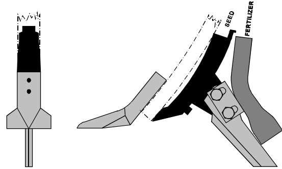
Figure 1. Key Ag Four Inch Chrome With Backswept Knife.
