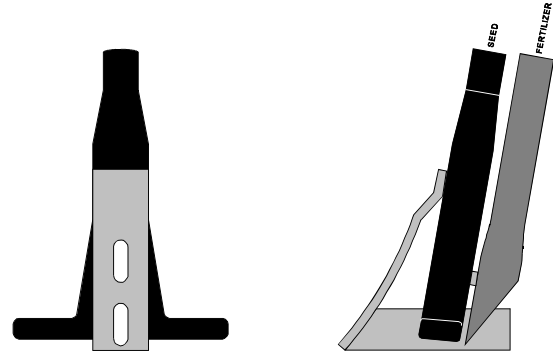
Figure 1. New Noble Seed-o-vator System.
