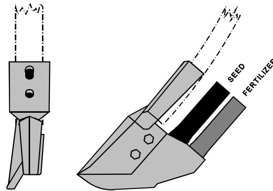
Figure 1. Swede Dual Placement Opener.
