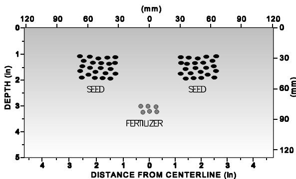
Figure 2. Seed and fertilizer placement.
