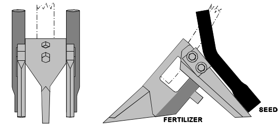
Figure 1. Key Ag Ventures Key Two Seeding System.
