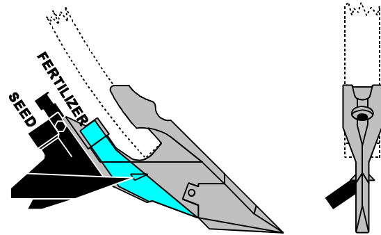
Figure 1. Flexi-coil Side Band Double Shoot Knife Opener.
