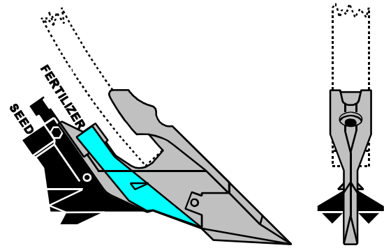
Figure 1. Flexi-coil HS Paired Row Double Shoot Knife Opener.
