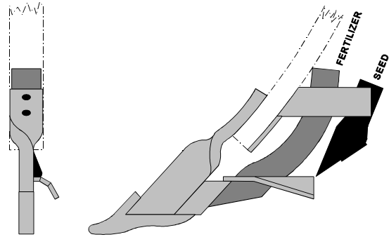
Figure 1. Morris Conventional Double Shoot Opener.
