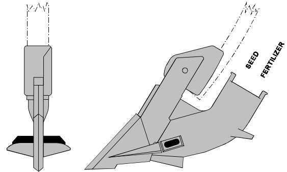
Figure 1. GEN 200 T2X2 Seeding System.
