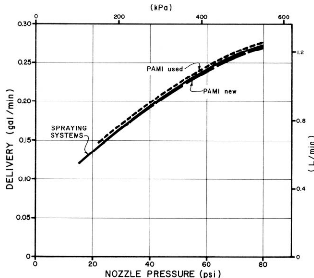
FIGURE 5. Delivery Rates for TeeJet 730231 Brass Nozzles.
