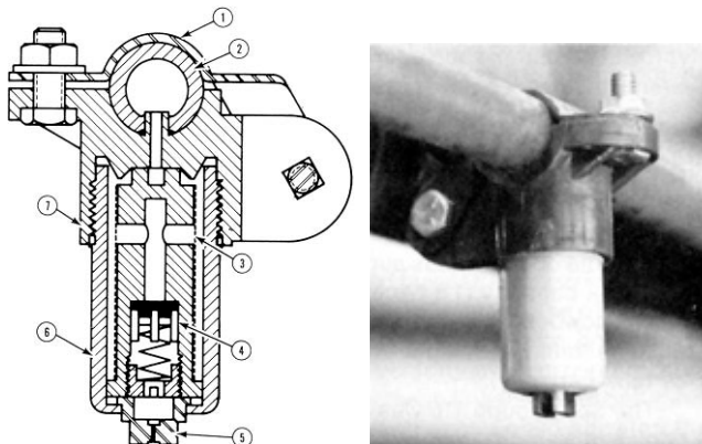
FIGURE 6. Cross Section of Nozzle Assembly: (1) Clamp Top, (2) Spray Boom, (3) Strainer, (4) Check Valve, (5) Nozzle Tip, (6) Nozzle Cap, (7) Nozzle Body.
