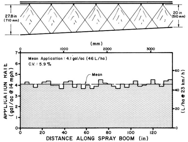
FIGURE 10. Typical Distribution Pattern along the Boom at 45 psi (300 kPa) Operating on a Sidehill, with the Boom Height Raised to Improve Distribution Uniformity.
