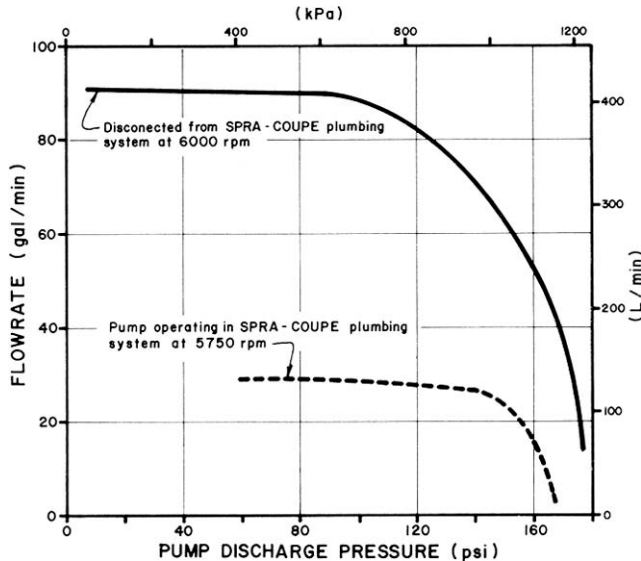
FIGURE 11. Pump Performance Curves.
