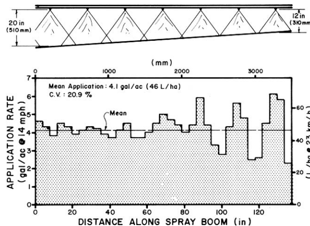
FIGURE 9. Typical Distribution Pattern along the Boom at 45 psi (300 kPa) when Operating on a Sidehill.
